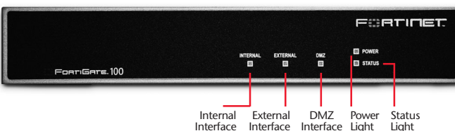
FortiGate-100
